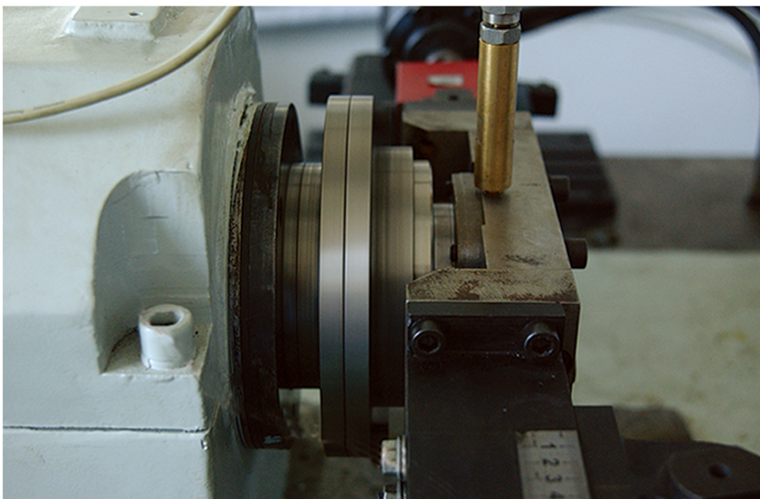
Hub Assembly Performance Tester
